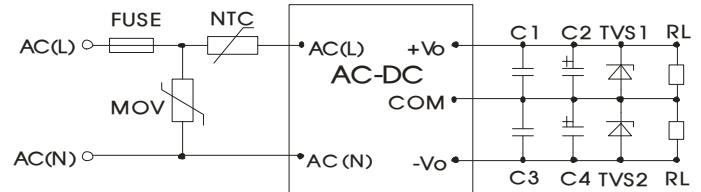
Fig. 2: LH40-10Axx typical application circuit
